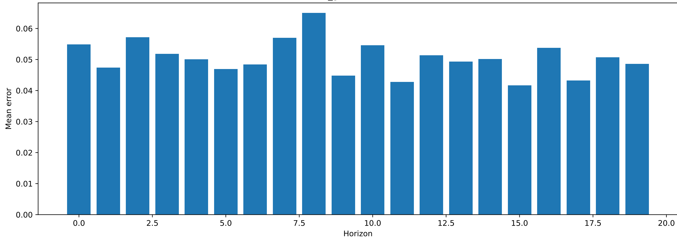
Test 1 MAE of default_gamma : 0.05048611760139465
