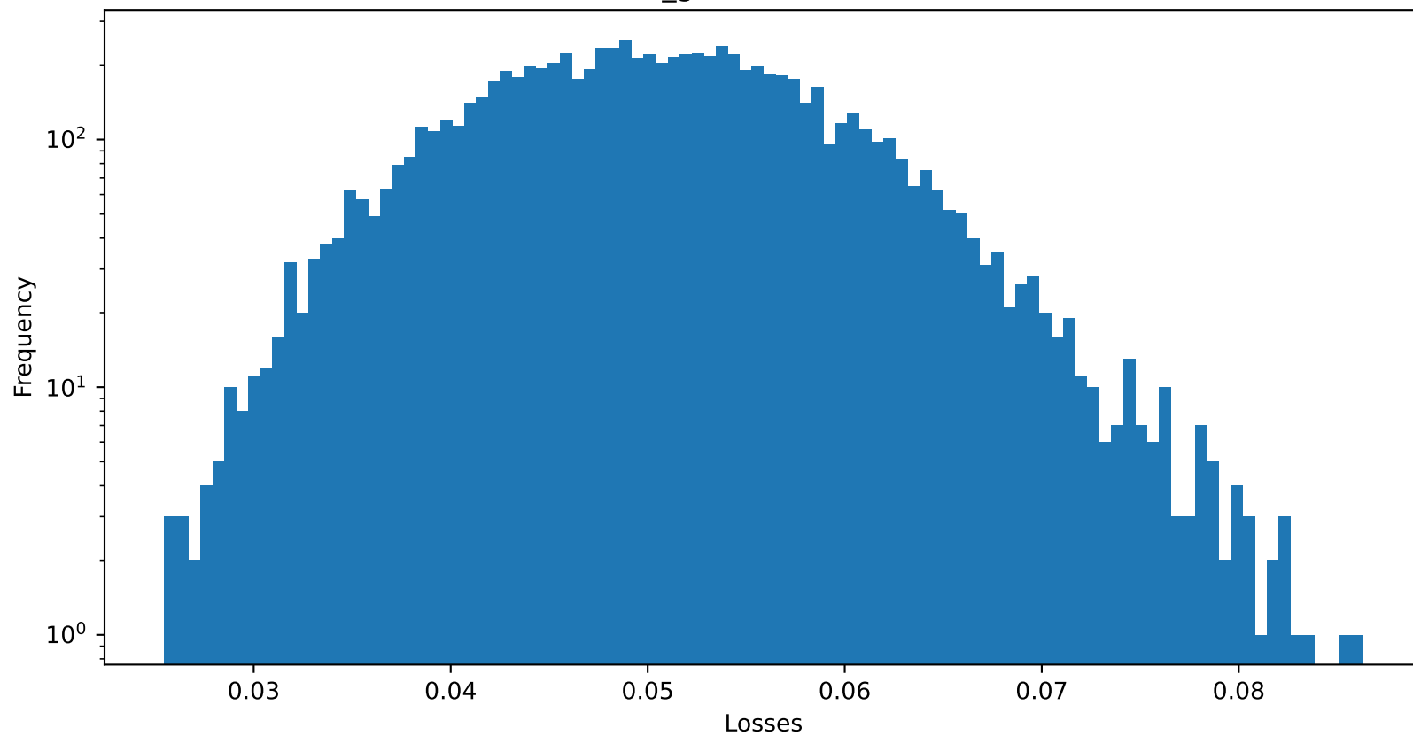
Test 2 MAE of default_gamma : 0.050532422959804535
