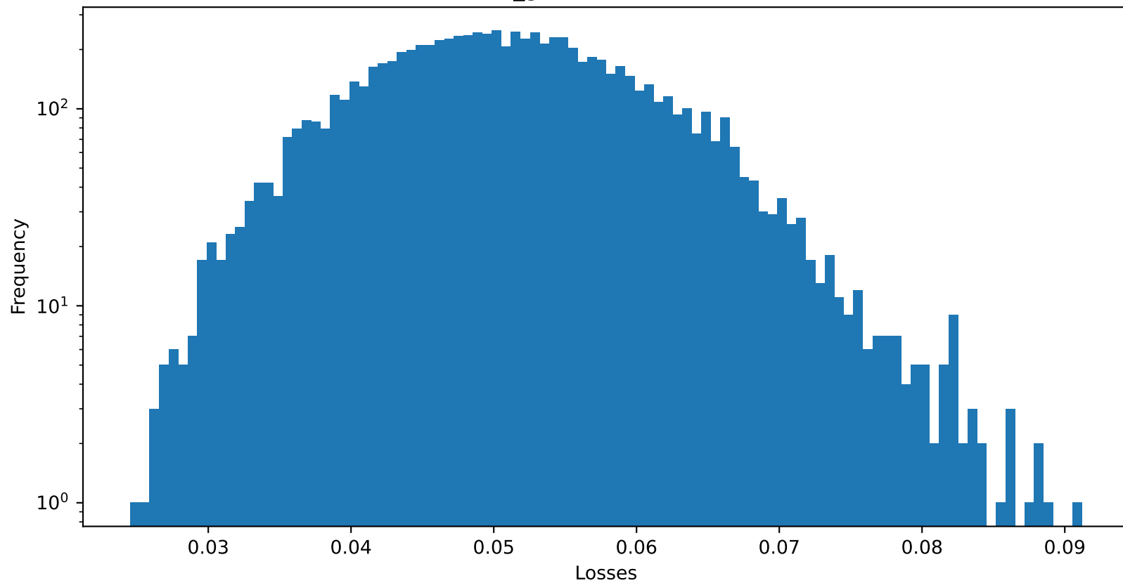
Test 2 MAE of fixed_gamma : 0.051145948469638824
