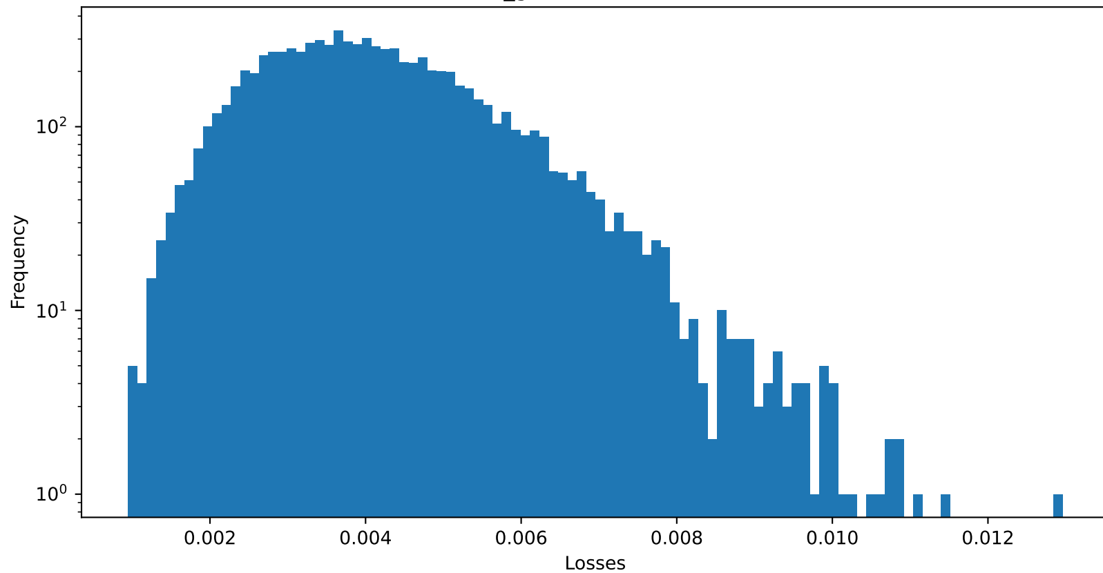
Test 2 MSE of fixed_gamma : 0.004117244388908148
