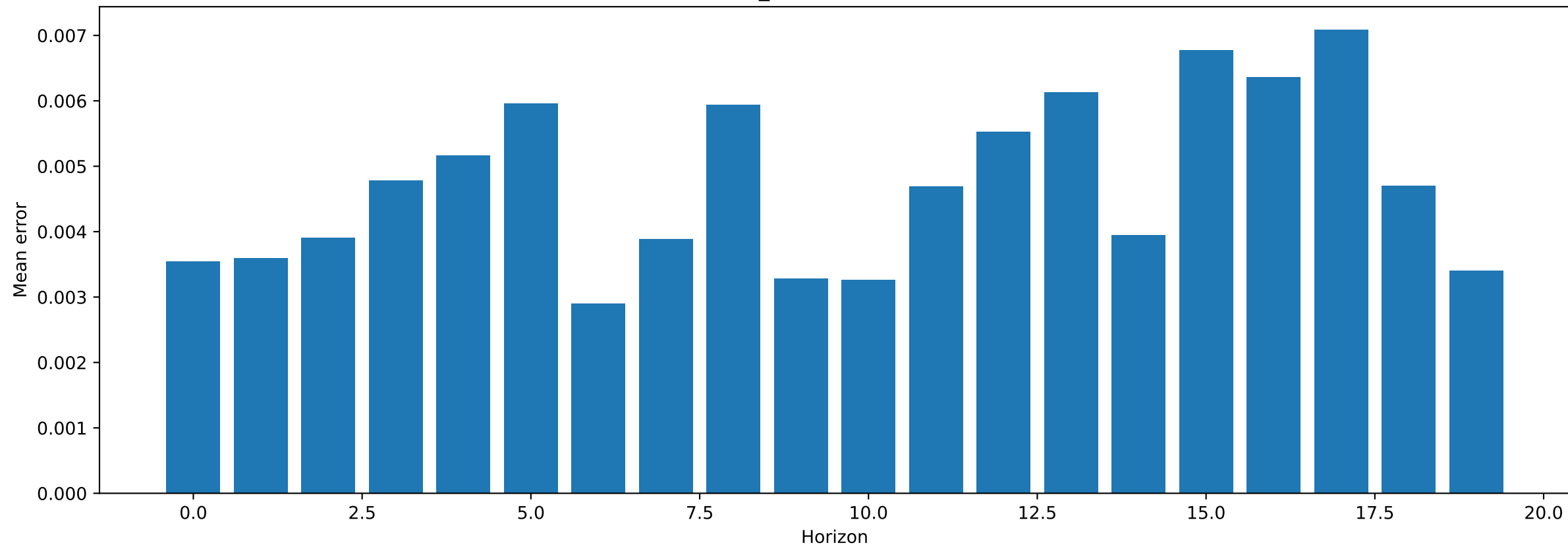
Test 2 MSE of PatchTST_instance : 0.0047437576577067375
