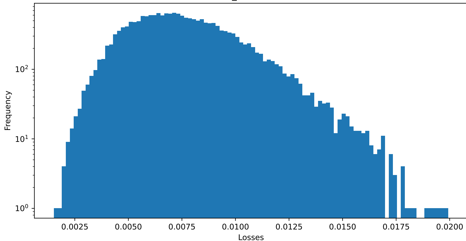
Test 1 NMSE of PatchTST_revin : 0.007607527542859316
