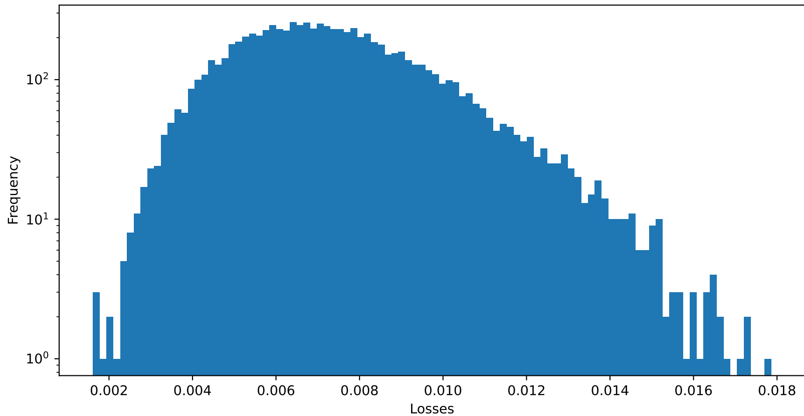
Test 2 NMSE of default : 0.007442583329975605
