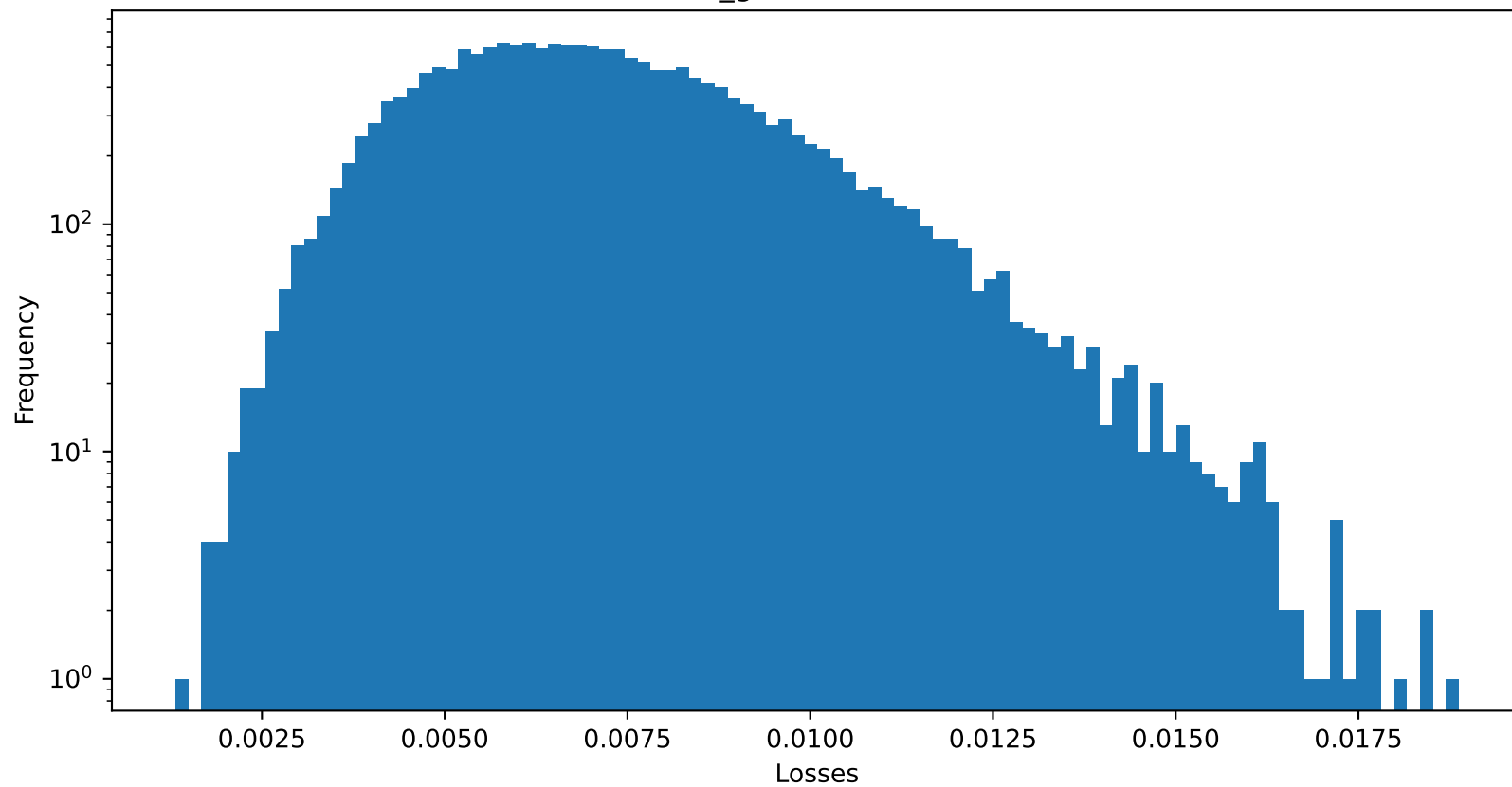
Test 1 NMSE of default_gamma : 0.007191733922809362
