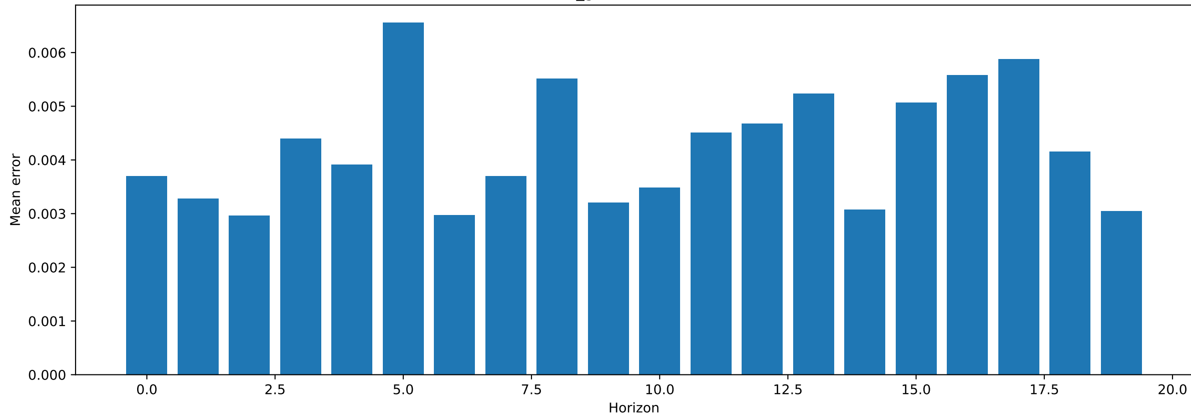
Test 1 MSE of default_gamma : 0.004247401375323534
