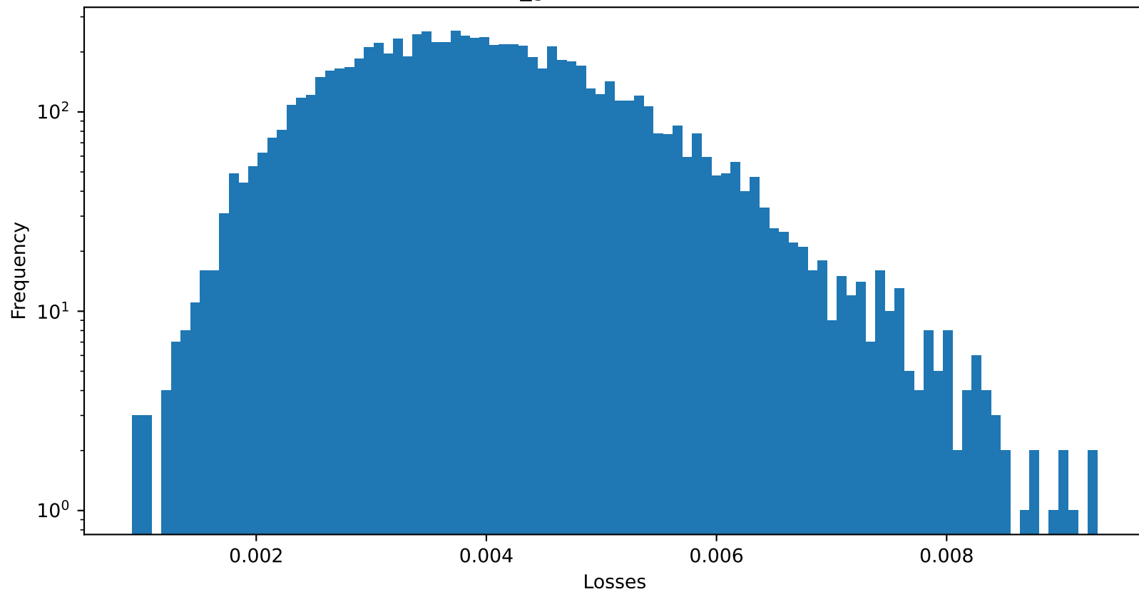
Test 2 MSE of fixed_gamma : 0.004000791814178228
