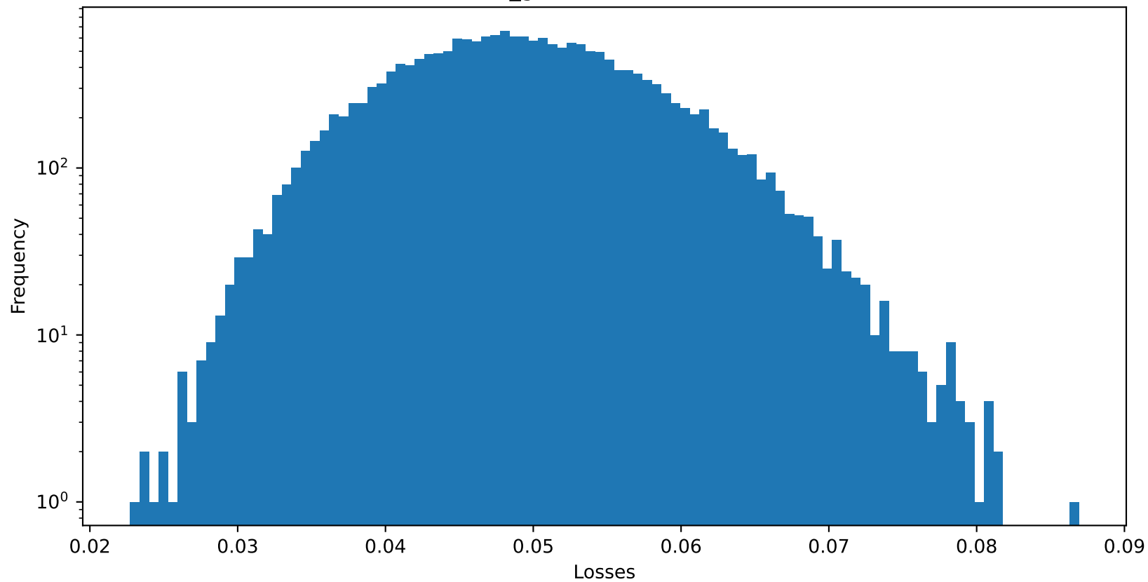
Test 1 MAE of init_gamma : 0.04940642789006233
