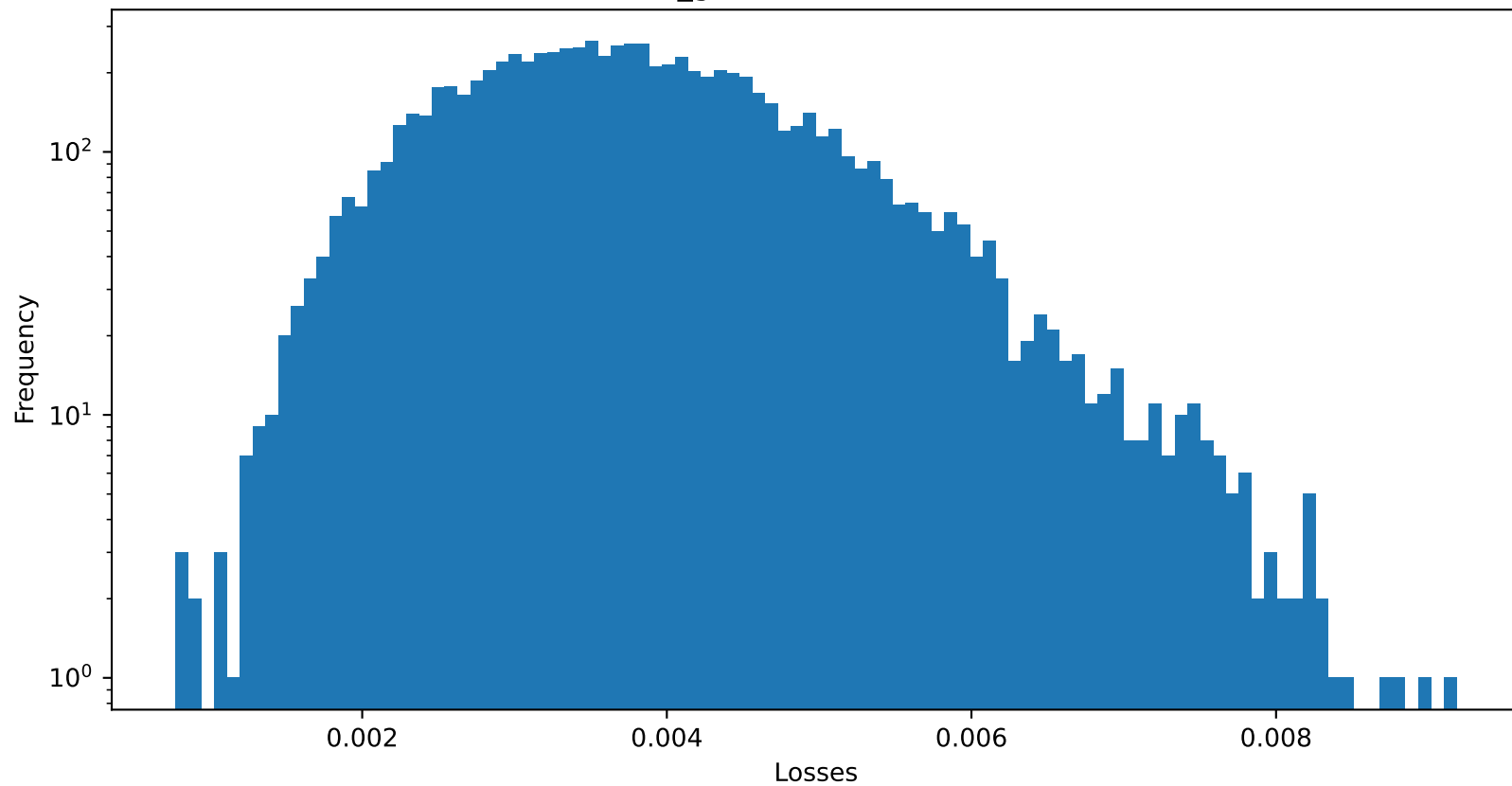
Test 2 MSE of init_gamma : 0.003819170640781522
