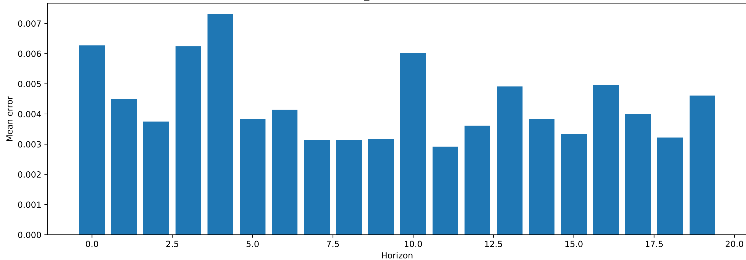
Test 1 MSE of PatchTST_instance : 0.004345266614109278
