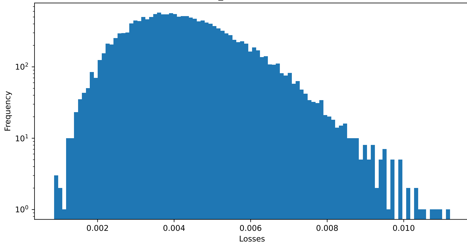
Test 2 MSE of PatchTST_instance : 0.0042638578452169895
