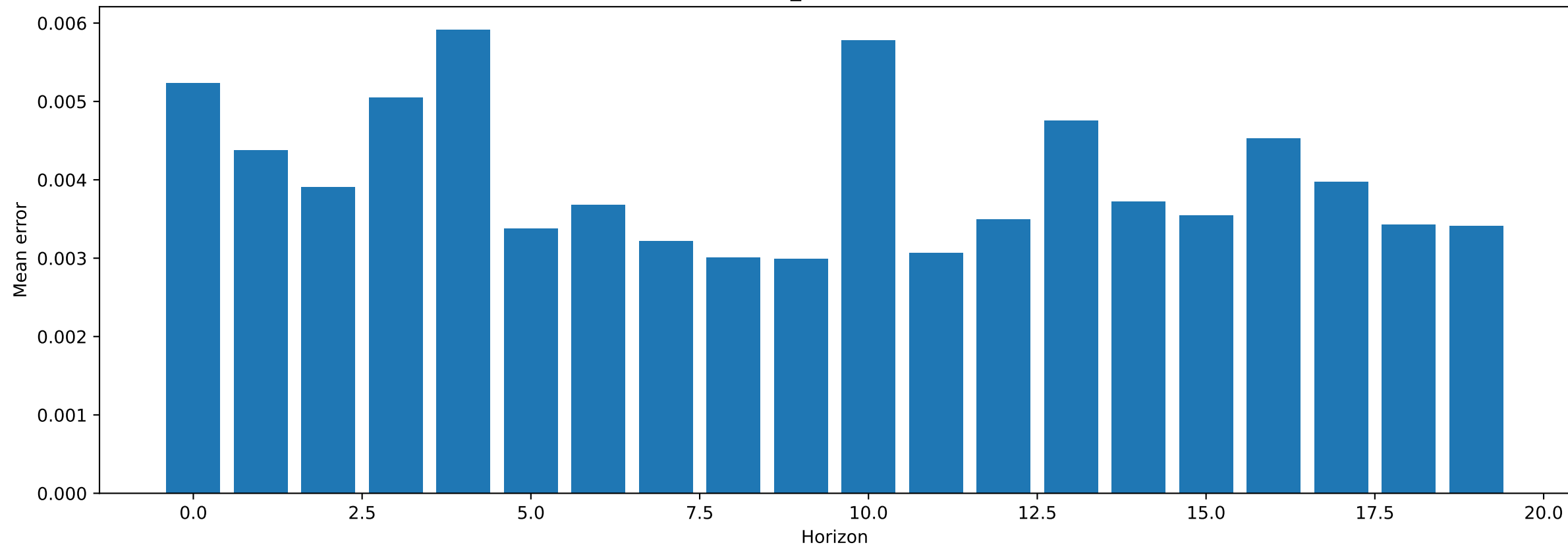
Test 1 MSE of PatchTST_revin : 0.00402422109618783
