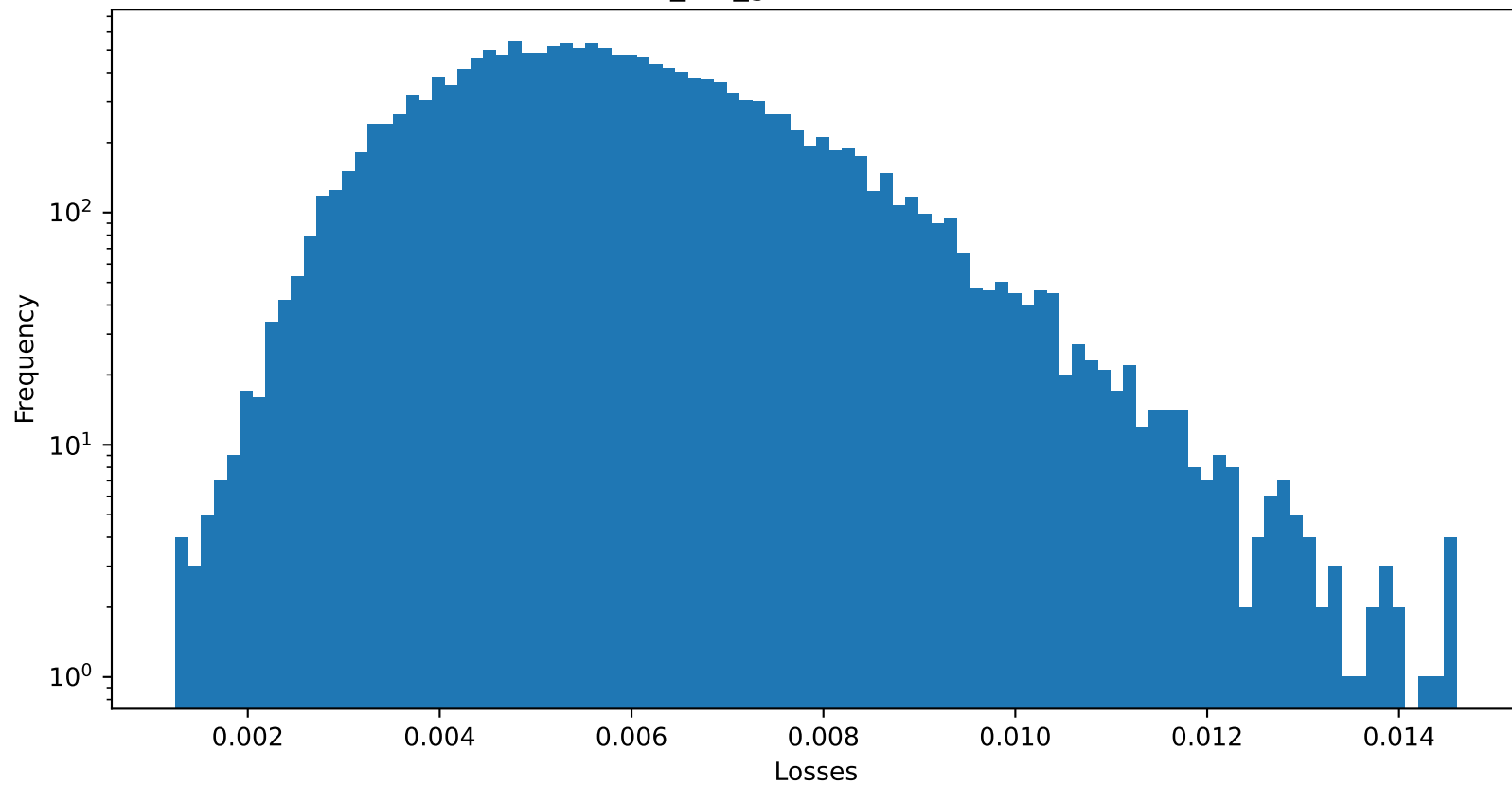
Test 2 NMSE of cmin_init_gamma : 0.005853950046002865
