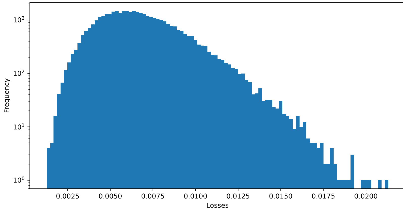
Test 1 NMSE of min : 0.006764634512364864
