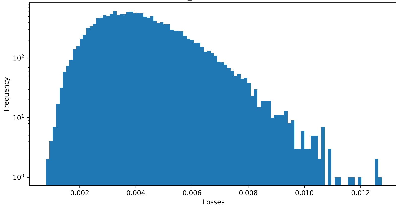
Test 2 MSE of PatchTST_instance : 0.004185592755675316
