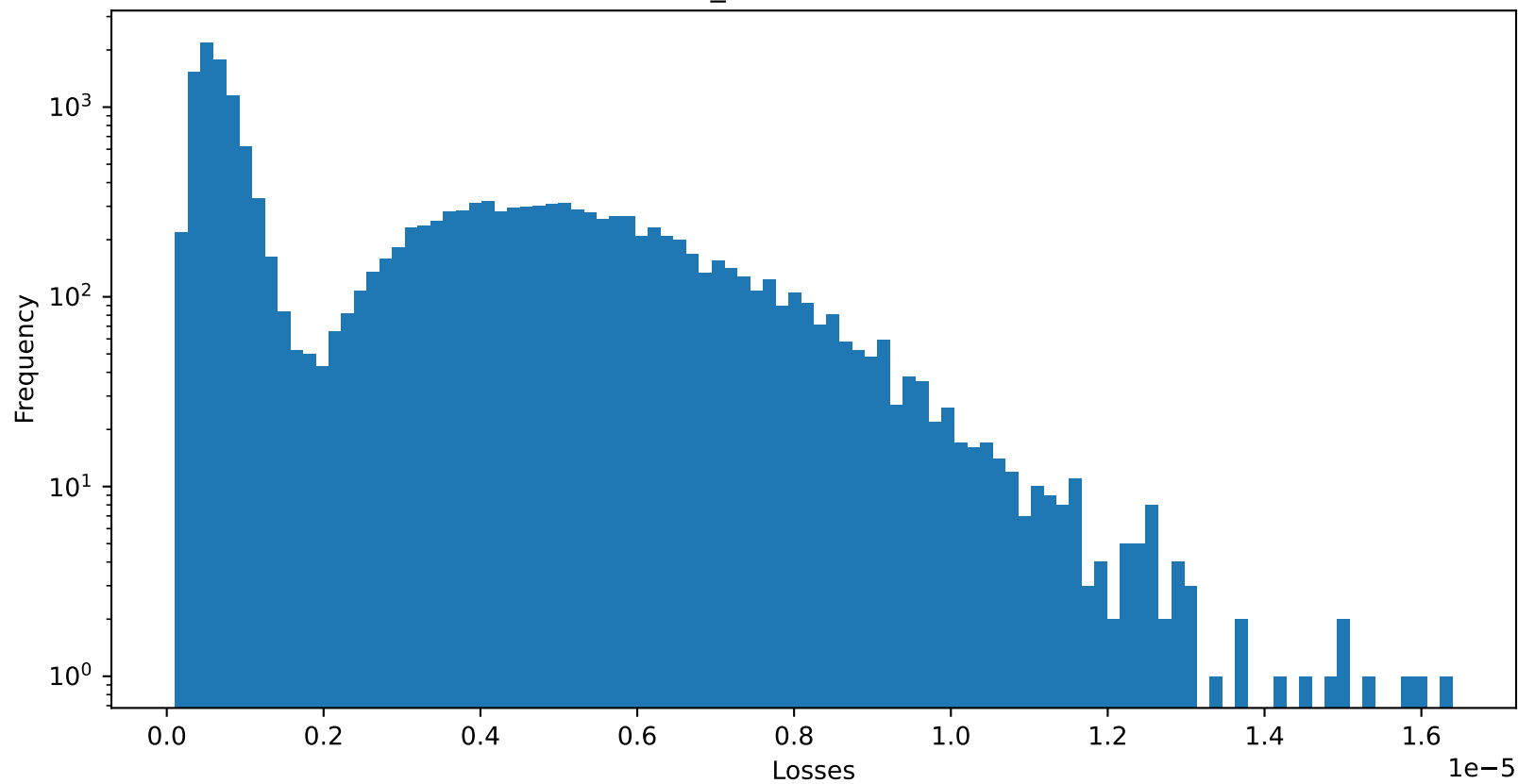
Test 2 RMSE of PatchTST_instance : 3.0613505259680096e-06
