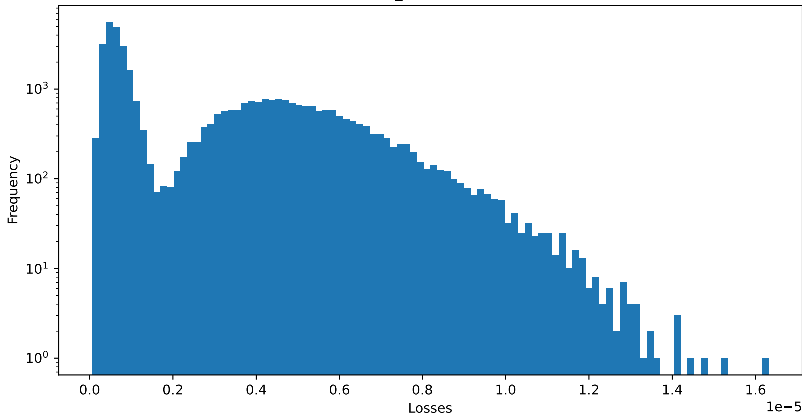
Test 1 RMSE of PatchTST_revin : 2.852506895578699e-06
