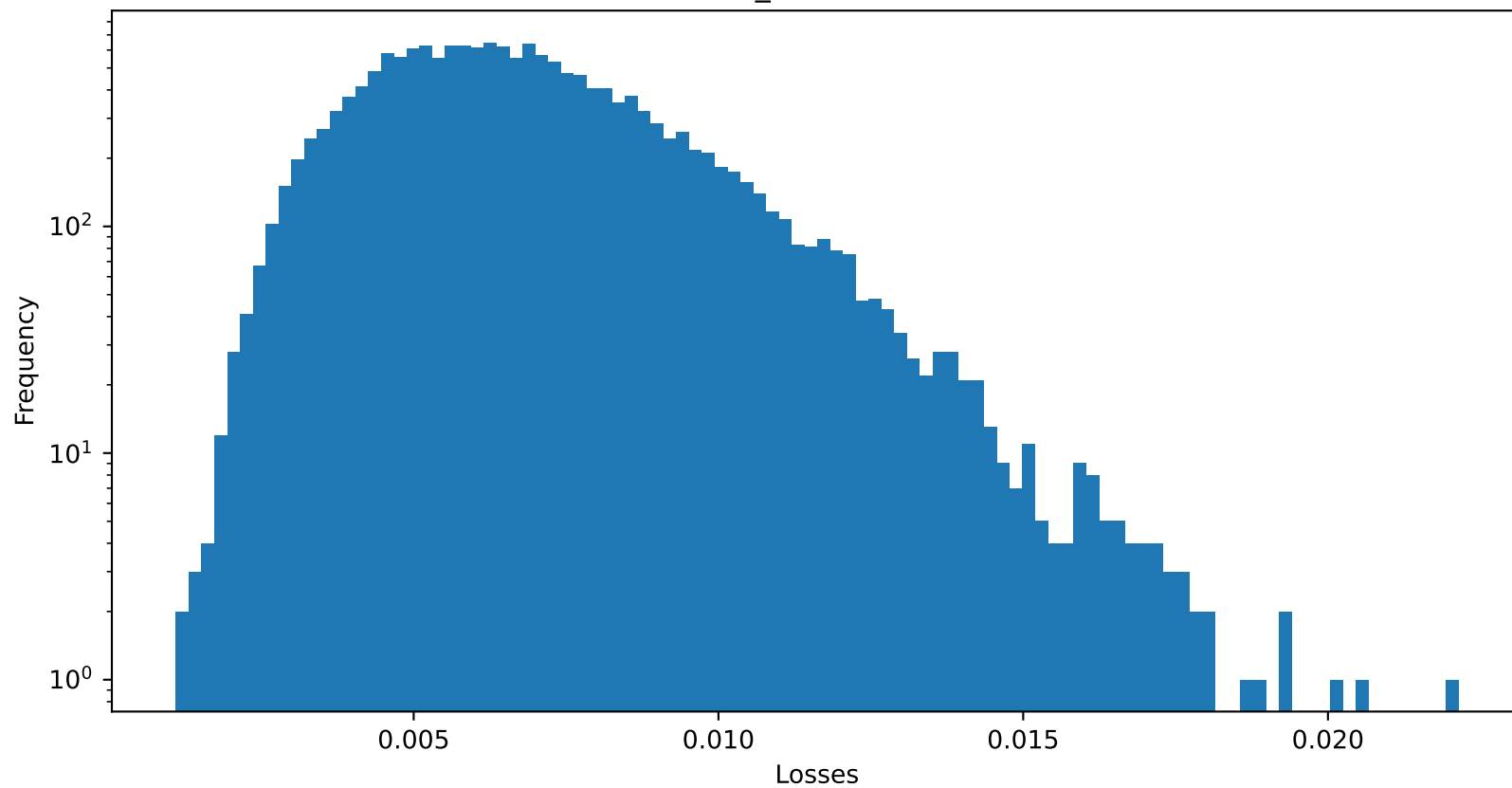
Test 2 NMSE of PatchTST_revin : 0.006759035401046276
