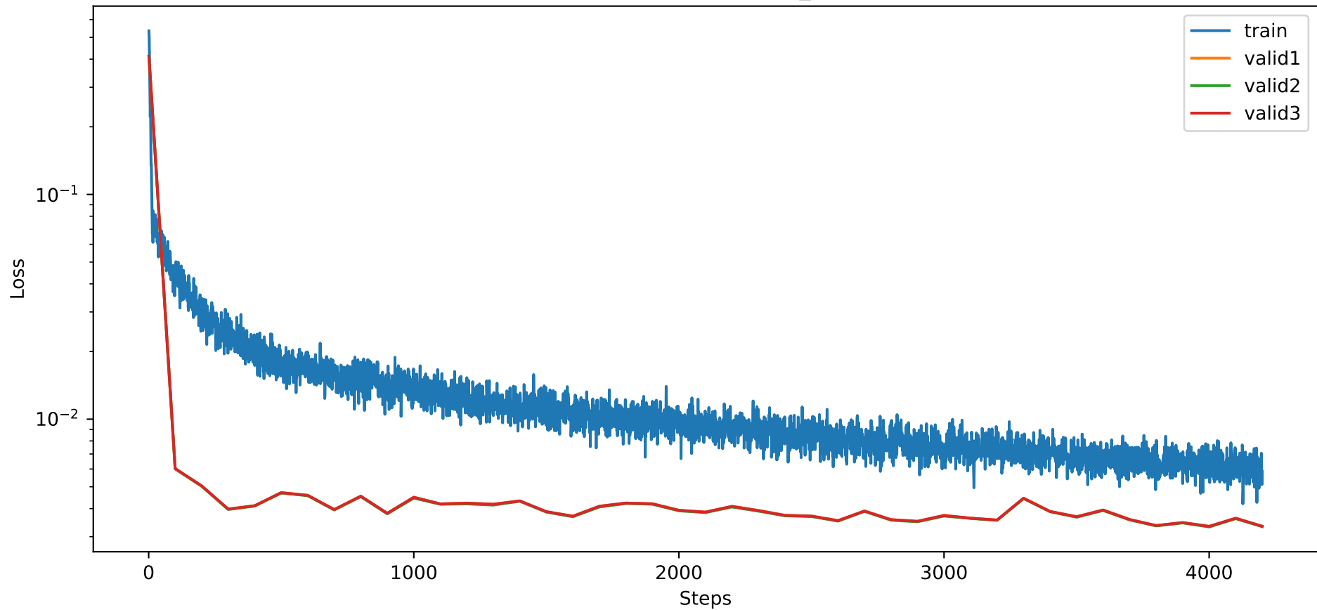
Training MSE of cmin_init
