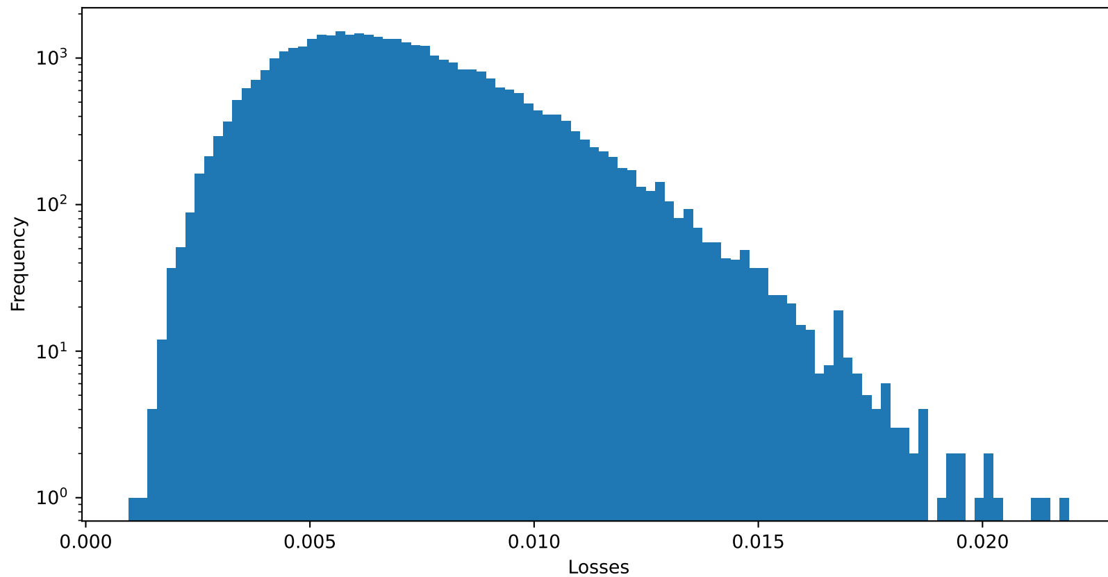
Test 1 NMSE of min : 0.006938524078577757
