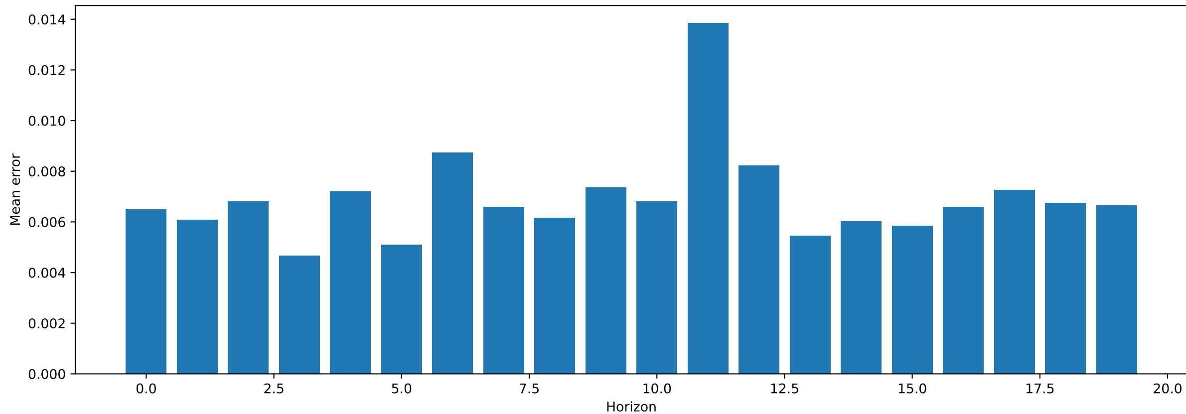
Test 1 NMSE of min : 0.006938524078577757
