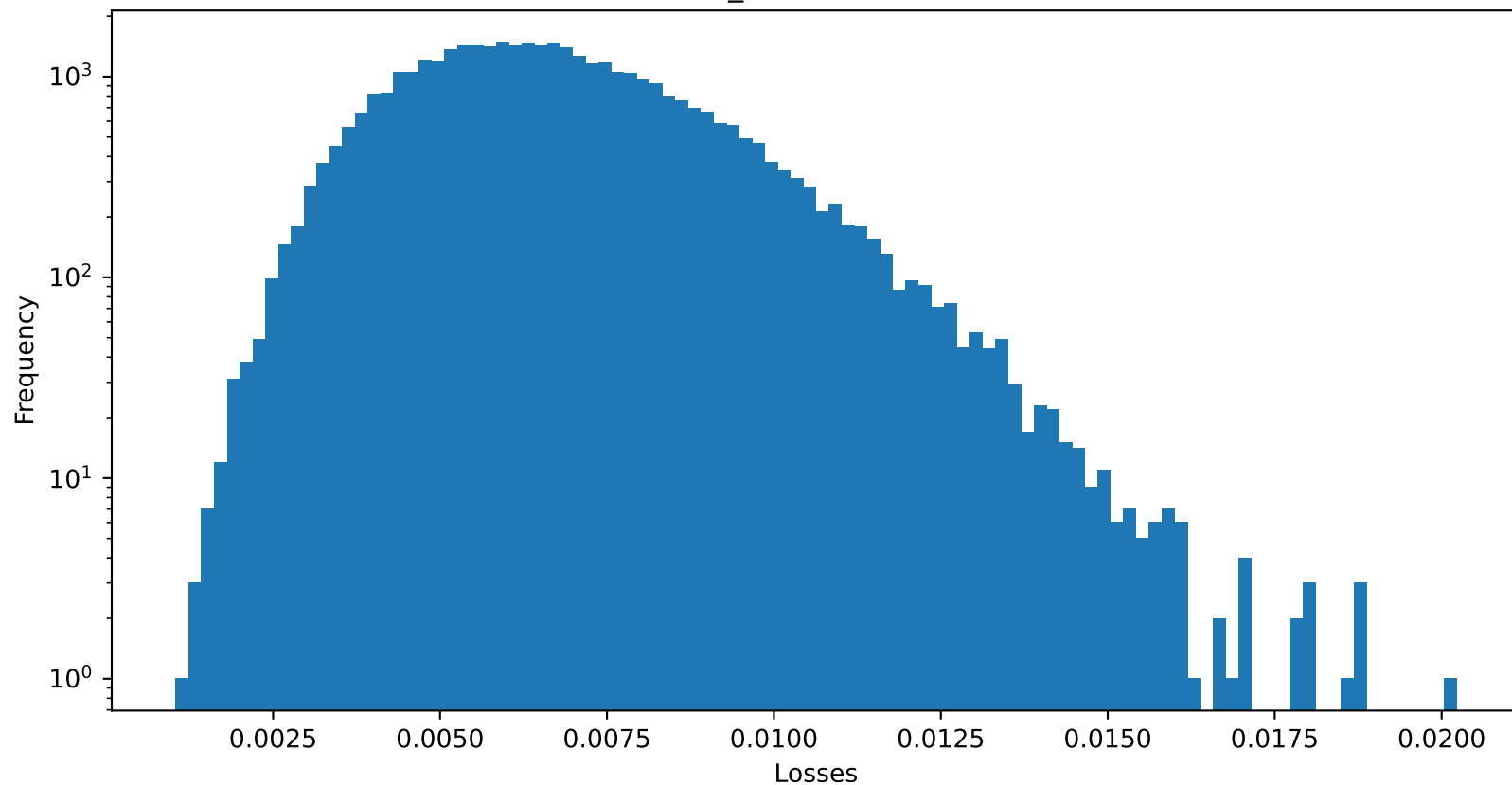
Test 1 NMSE of PatchTST_instance : 0.006715526804327965
