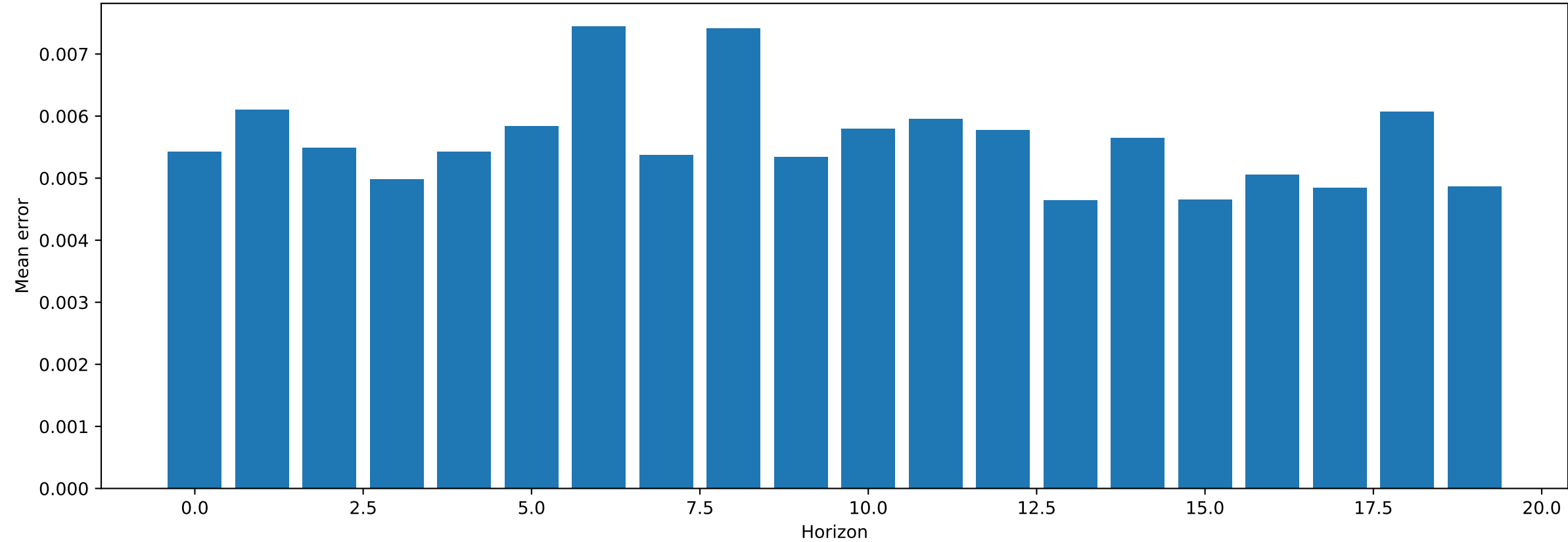
Test 1 NMSE of cmin_init : 0.0056092459708452225
