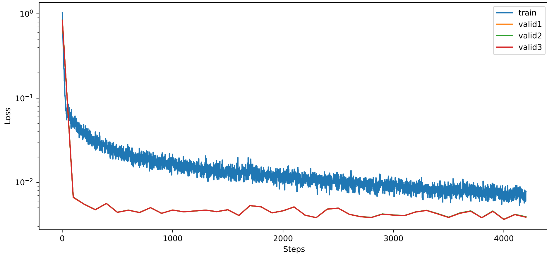
Training MSE of cmin_default
