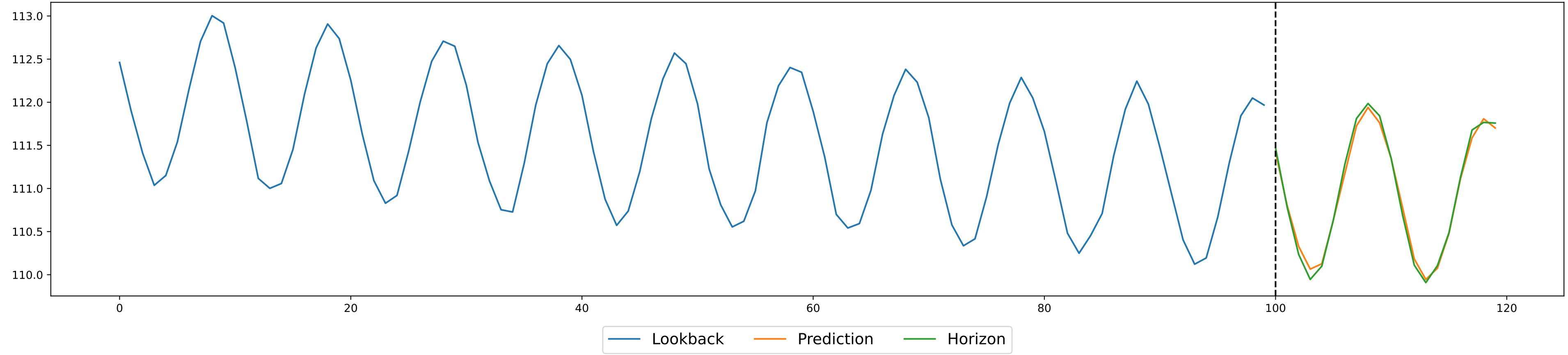
Example rand prediction for cmin_init_gamma
