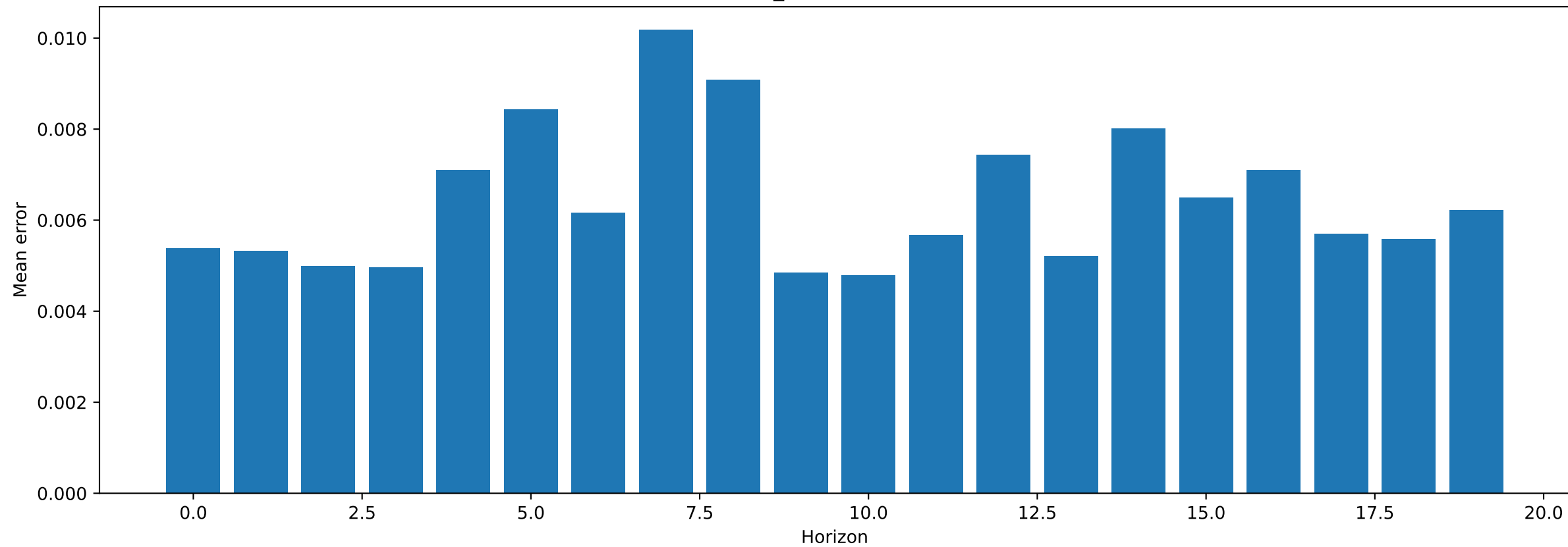
Test 2 NMSE of PatchTST_instance : 0.006436500232666731
