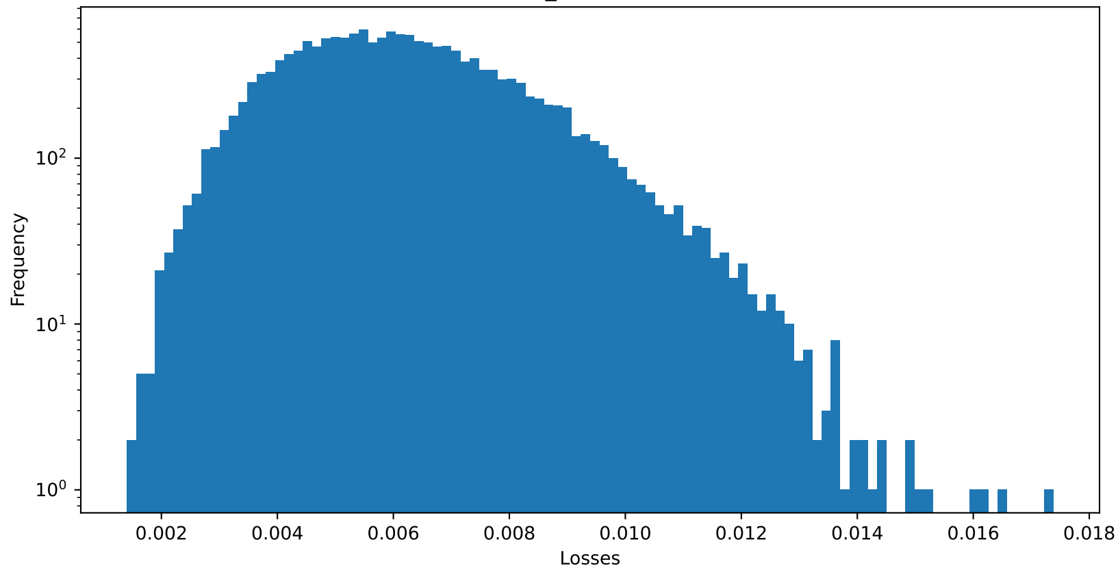
Test 2 NMSE of PatchTST_revin : 0.006205822806805372
