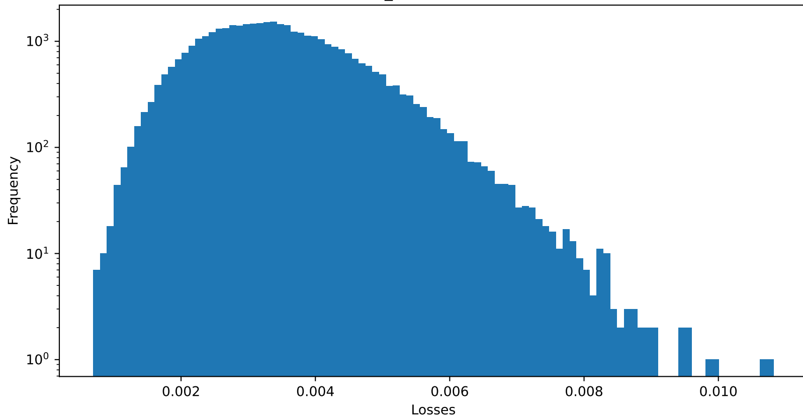
Test 1 MSE of cmin_init : 0.003459664760157466
