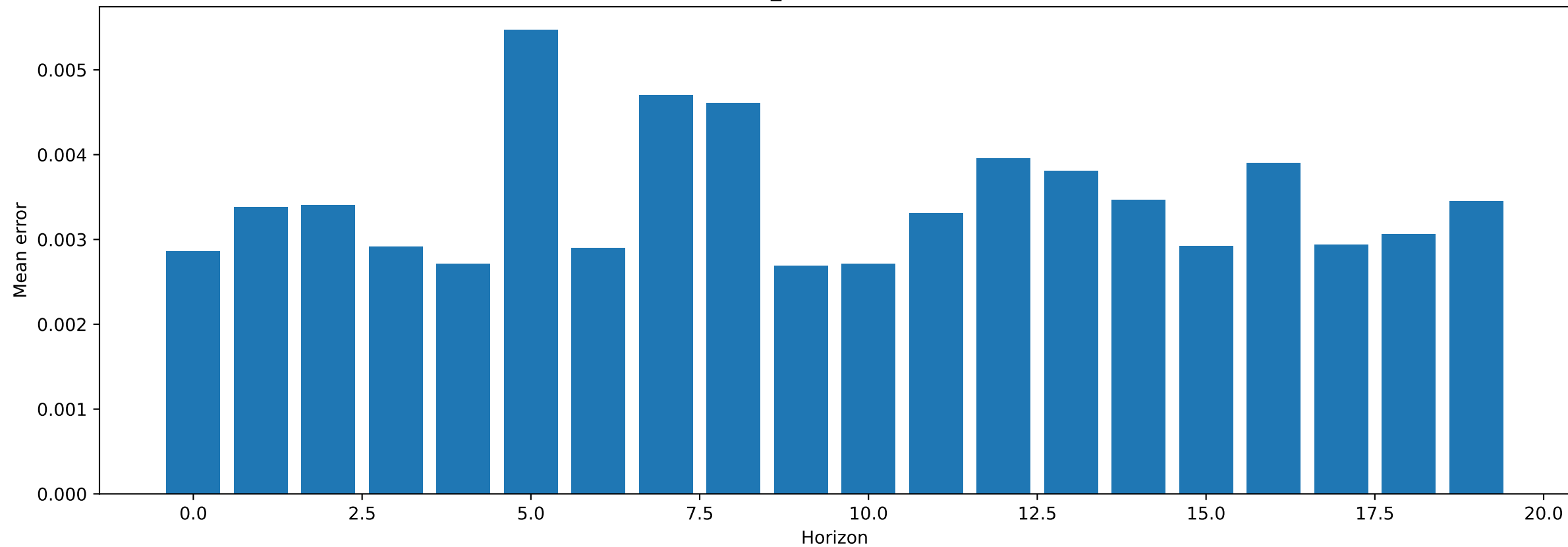
Test 1 MSE of cmin_init : 0.003459664760157466
