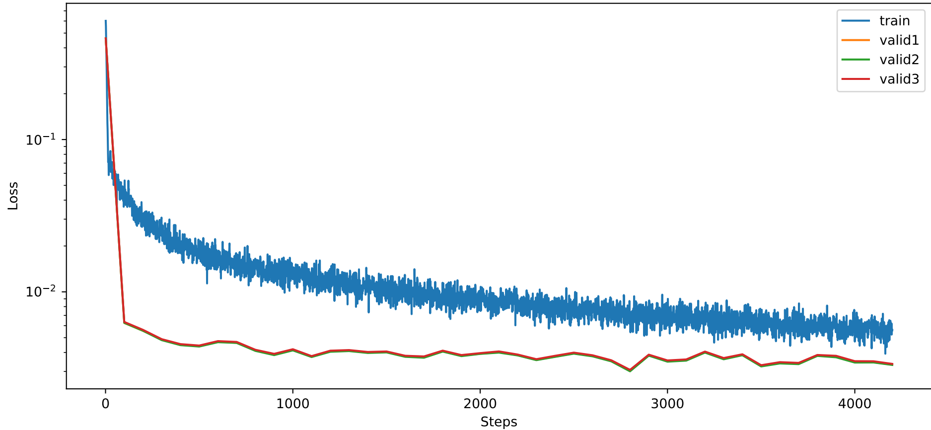
Training MSE of cmin_init_gamma
