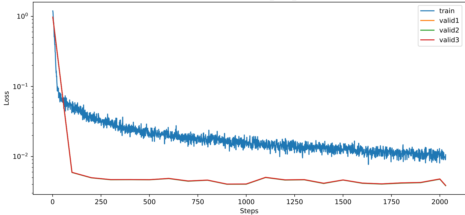
Training MSE of sim2_local_min
