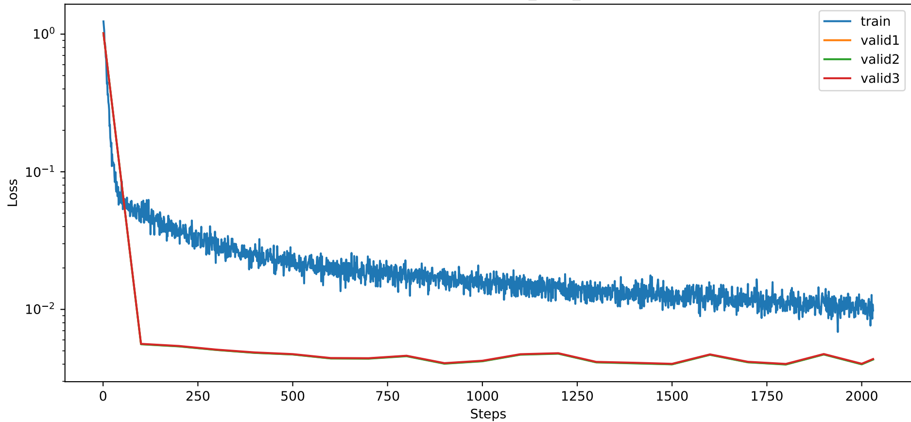
Training MSE of sim1_local_min
