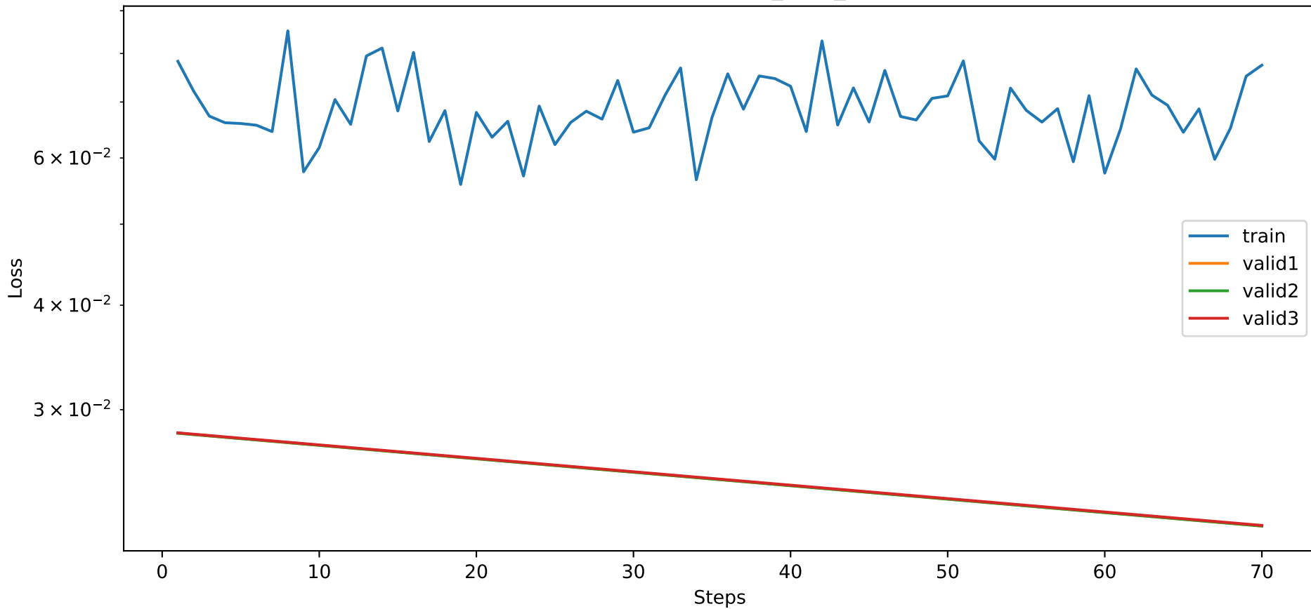
Training MSE of sim1_tune_revin
