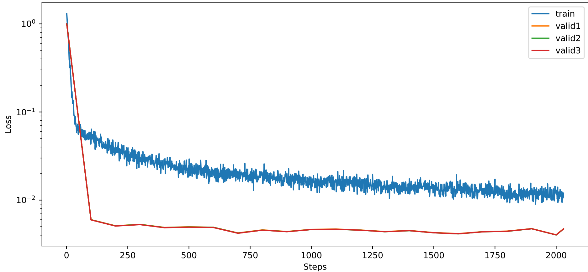
Training MSE of sim2_local_revin
