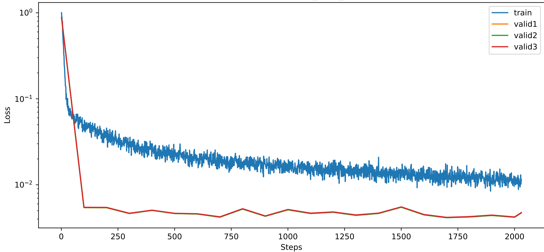
Training MSE of sim1_local_revin
