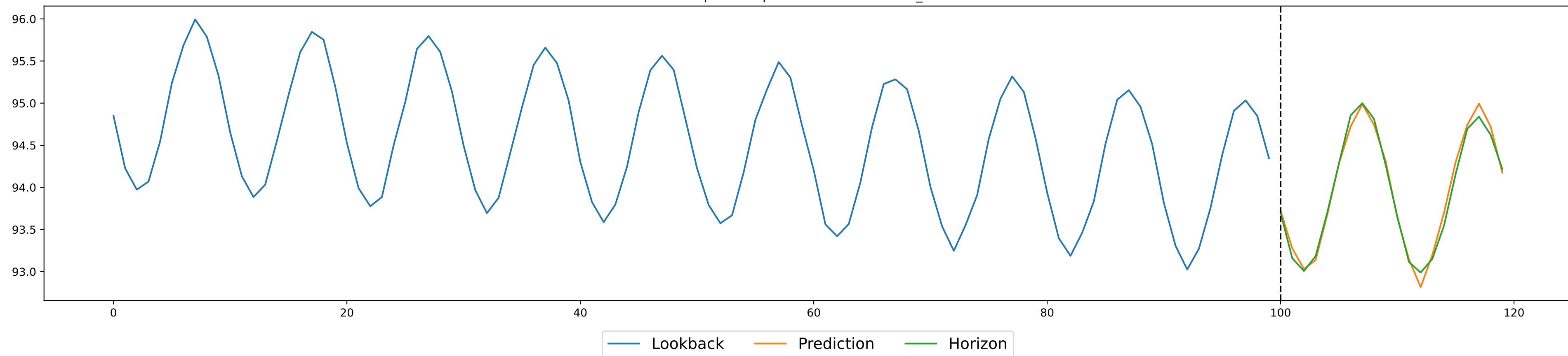
Example rand prediction for PatchTST_min
