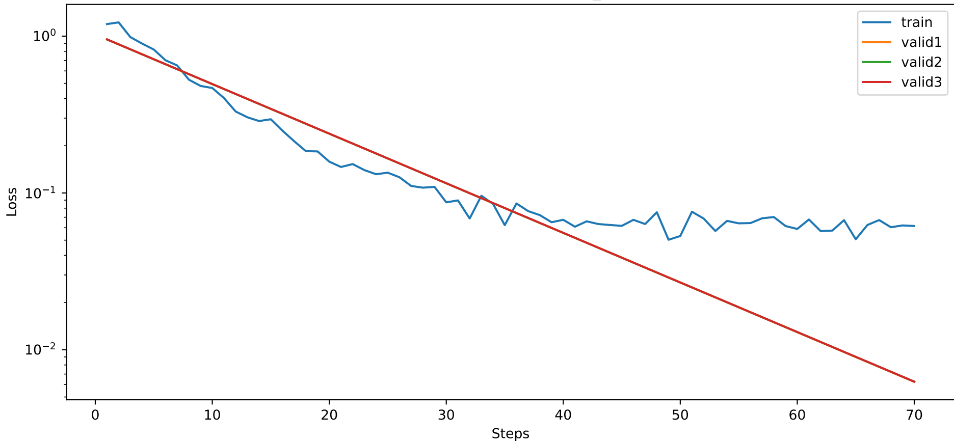
Training MSE of PatchTST_mIN
