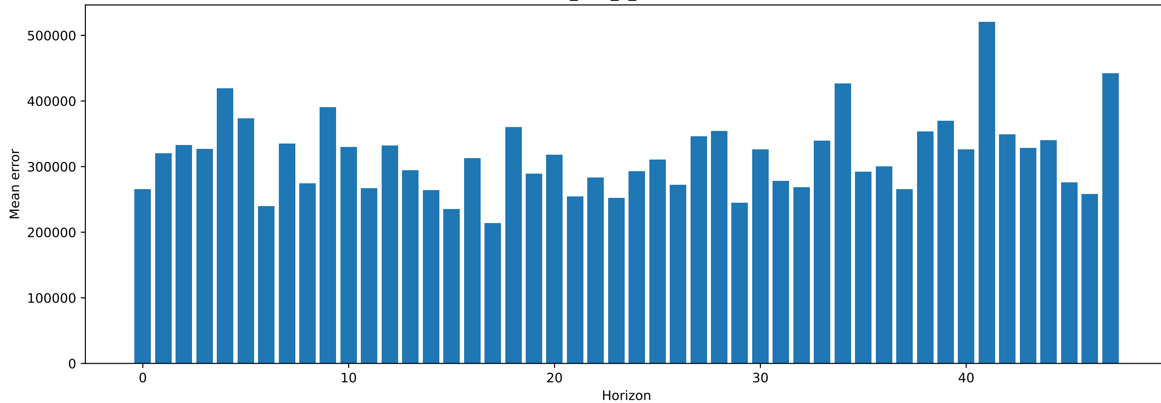
Test 2 MSE of PatchTST_MSE_2_removeFalse : 315970.40625
