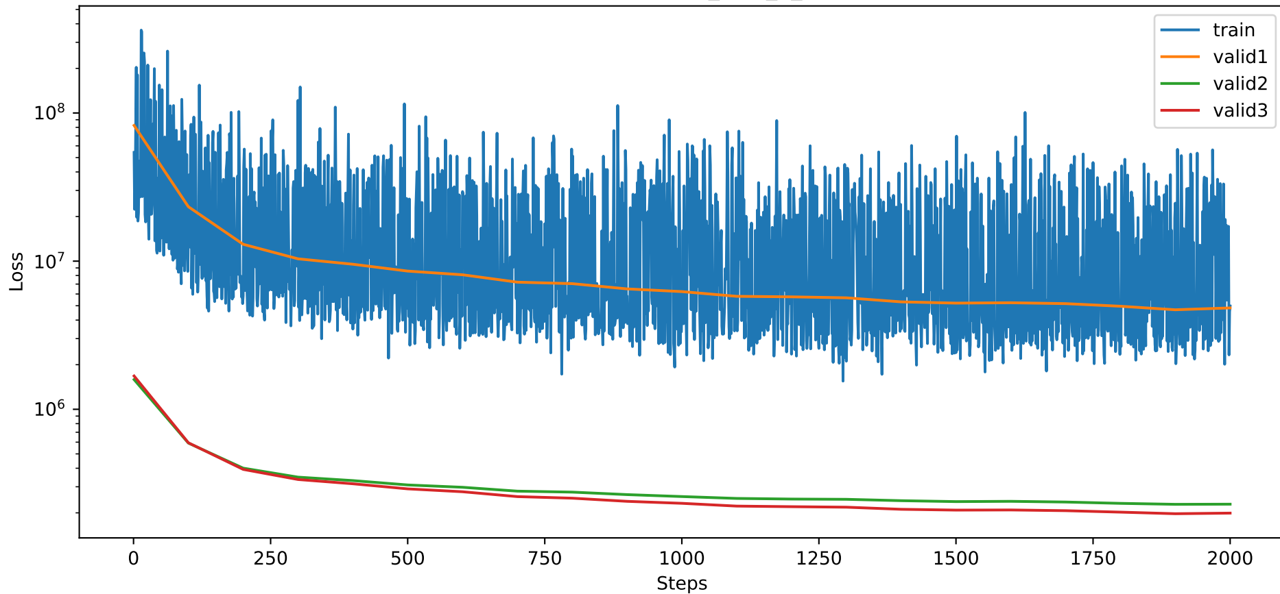
Training MSE of PatchTST_MSE_2_removeTrue
