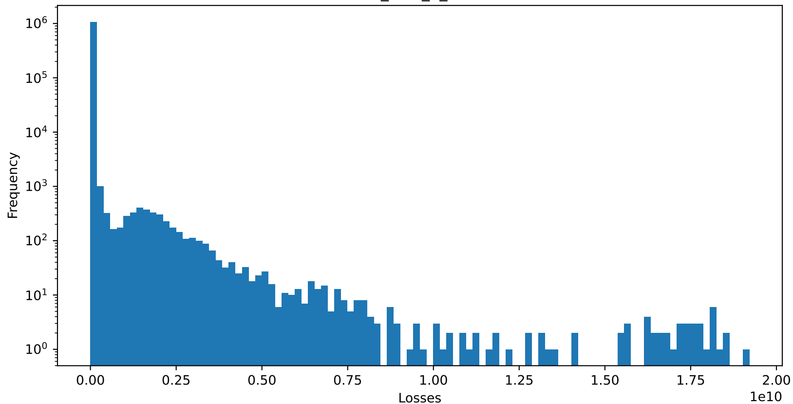
Test 1 MSE of PatchTST_MSE_2_removeTrue : 9736535.0
