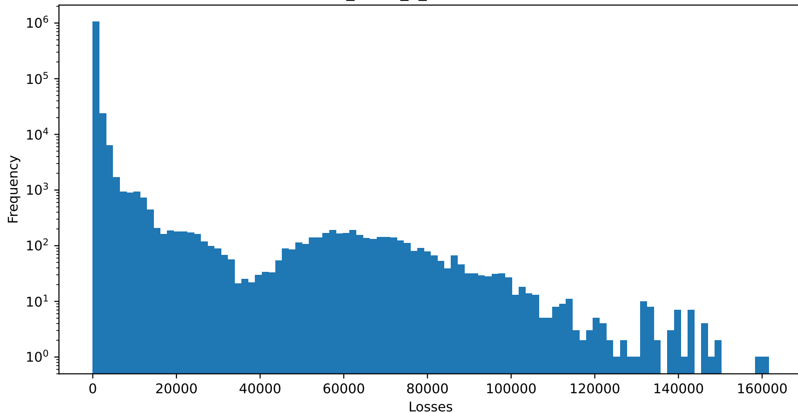
Test 1 MAE of PatchTST_NMSE_2_removeFalse : 564.567138671875
