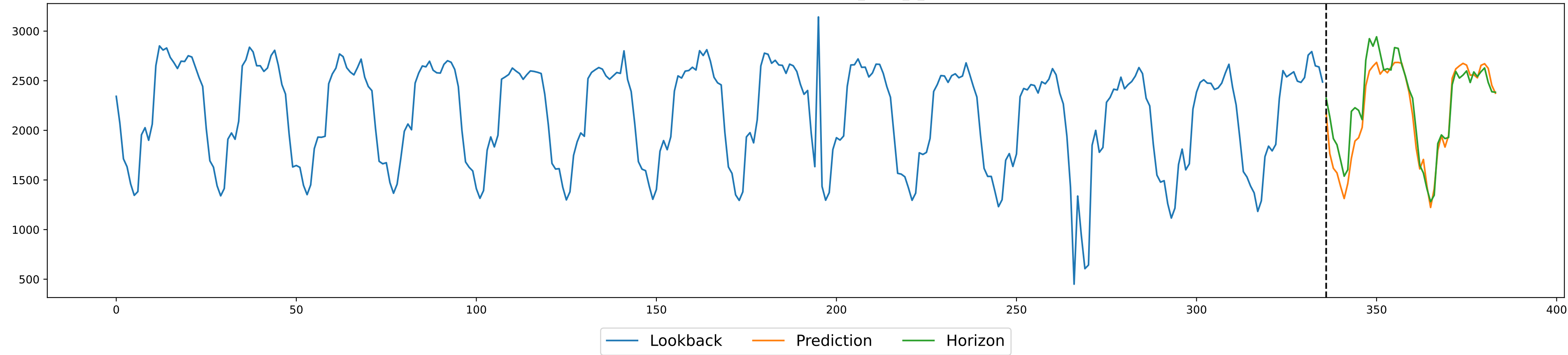
Example rand prediction for PatchTST_NMSE_2_removeTrue
