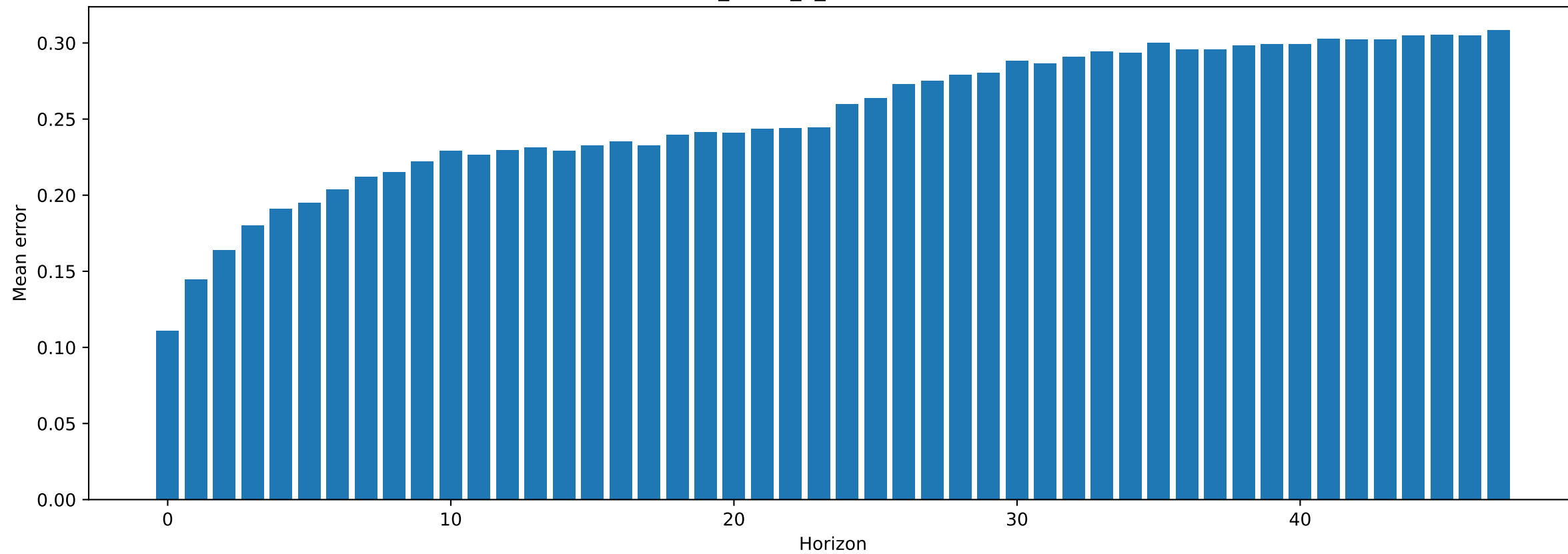
Test 1 NMSE of PatchTST_NMSE_2_removeTrue : 0.2530306577682495
