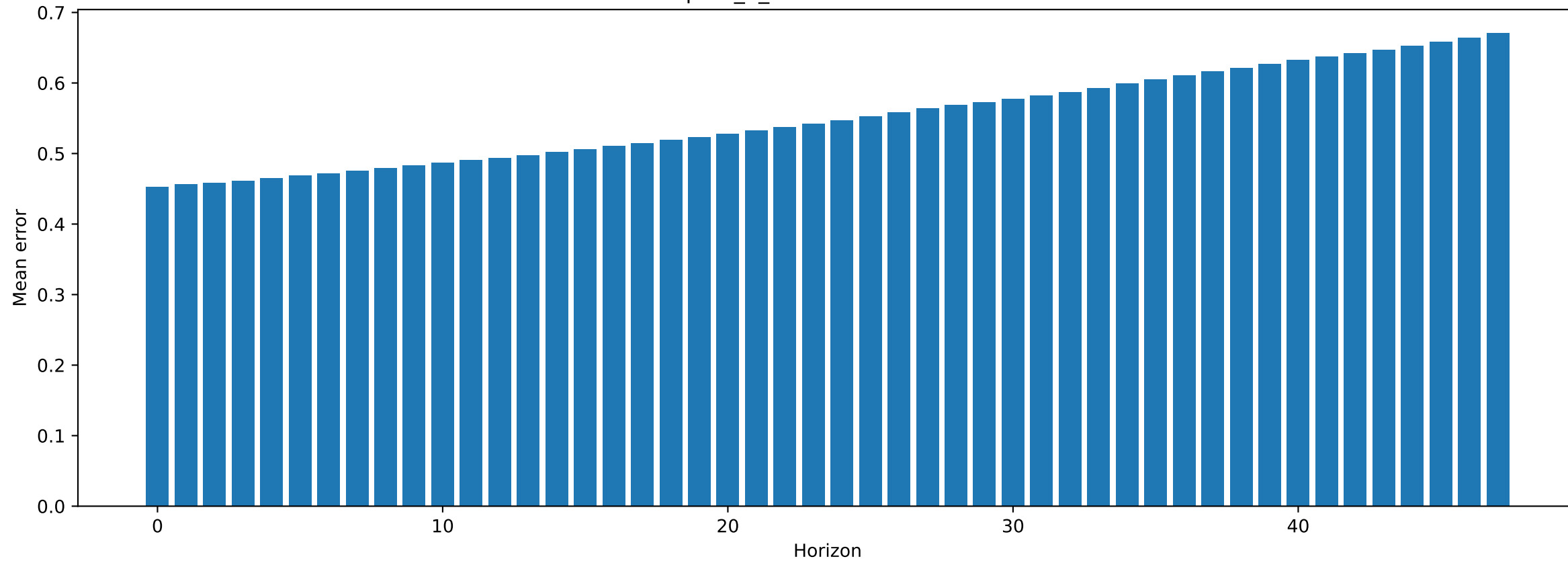
Test 2 NMSE of repeat_2_removeTrue : 0.5509858131408691
