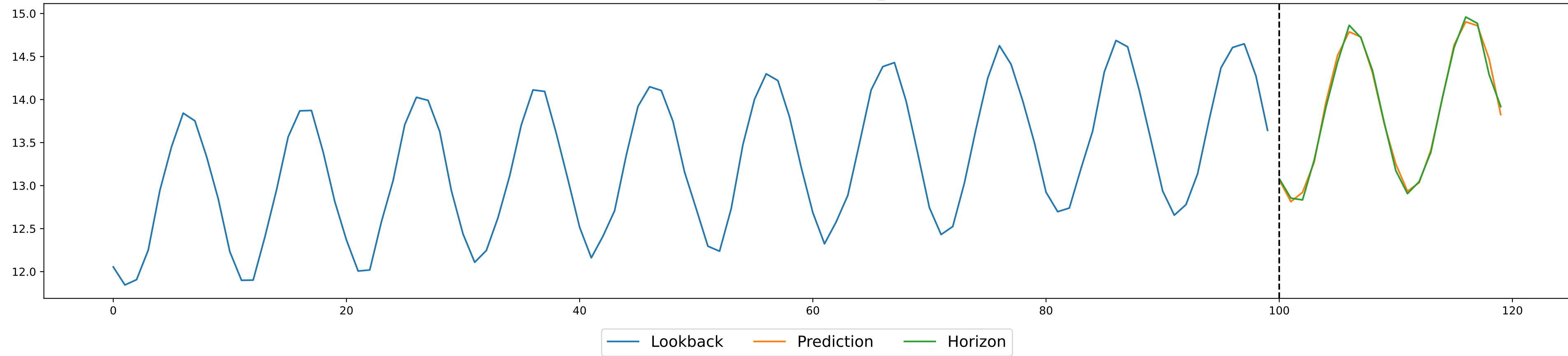
Example rand prediction for min_init+revin
