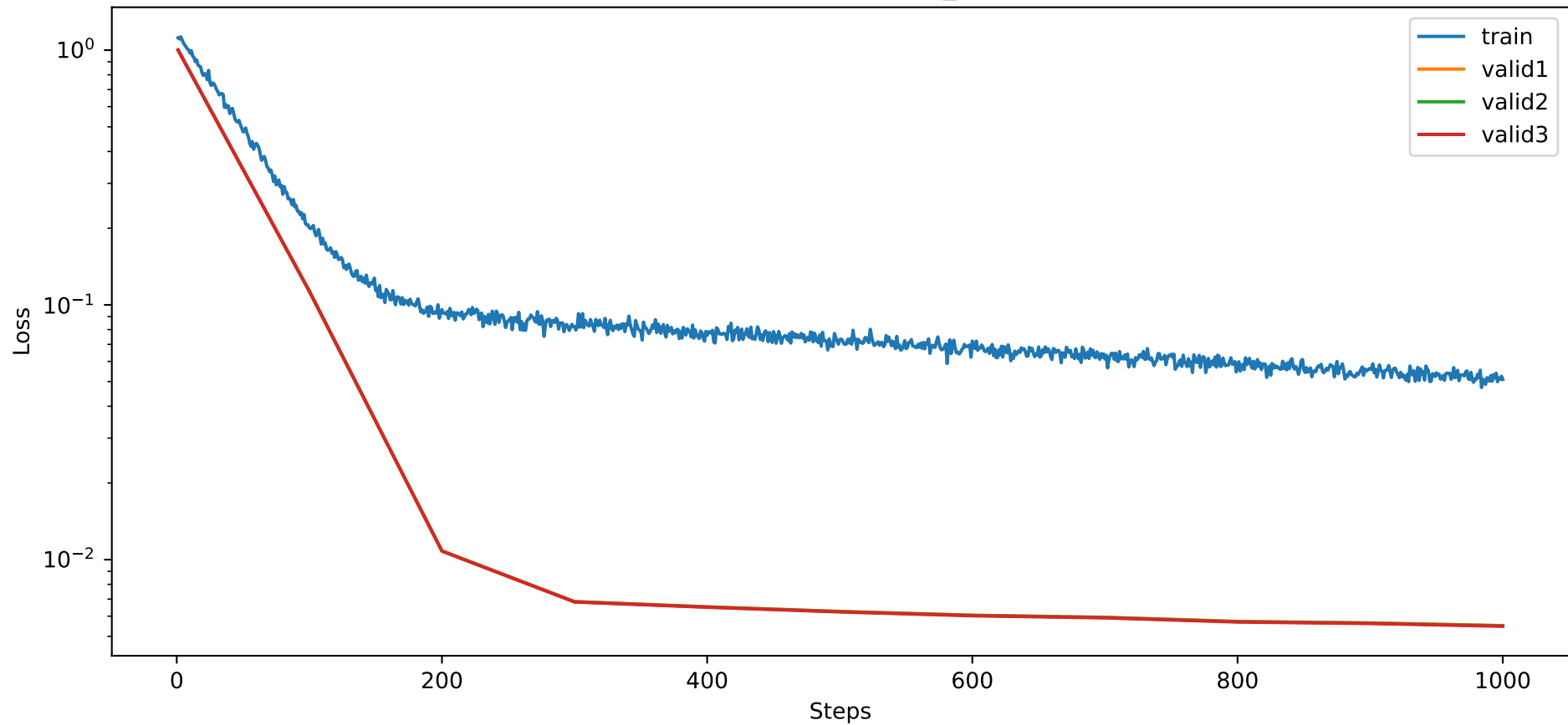
Training NMSE of min_fixed
