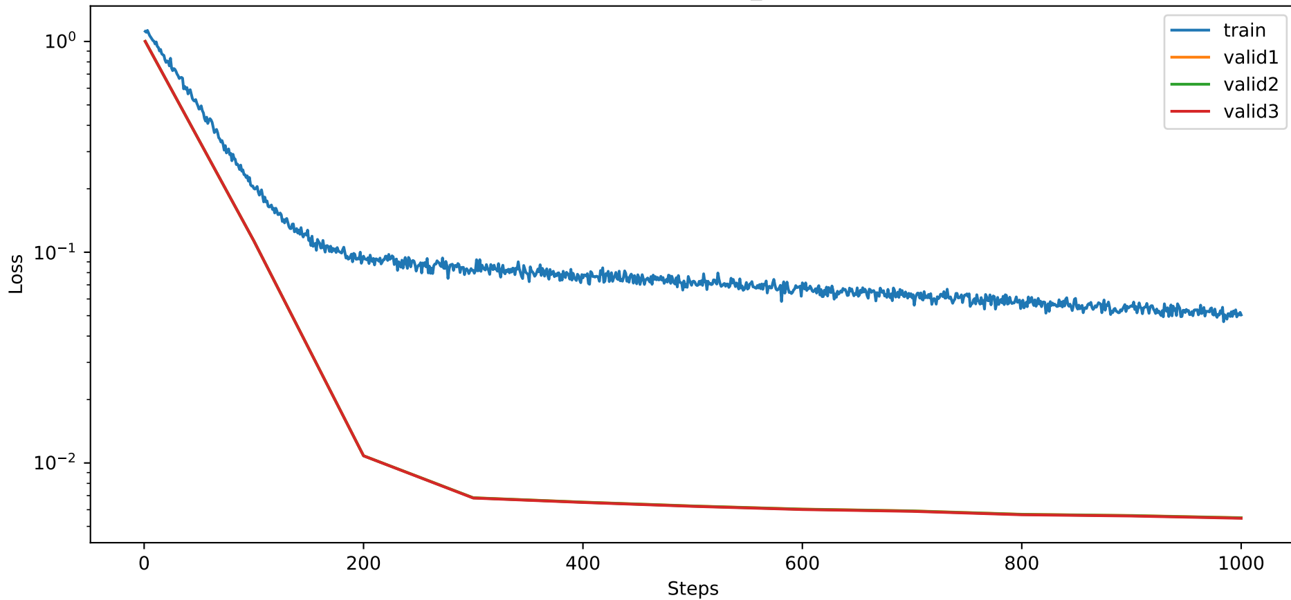
Training NMSE of min_init+revin
